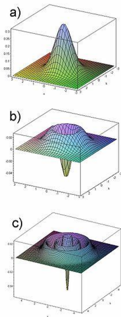
图 3.1 The Wigner quasi-probability distribution for a) the vacuum b) An n = 1 Fock state (e.g. a single photon) c) An n = 5 Fock state.
