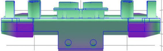
Fig. 9. Simulated resonant modes of the upper part of the system. The solid blue lines in the figure are the original position of the upper part. The darker the color, the greater the displacement of the upper part.
