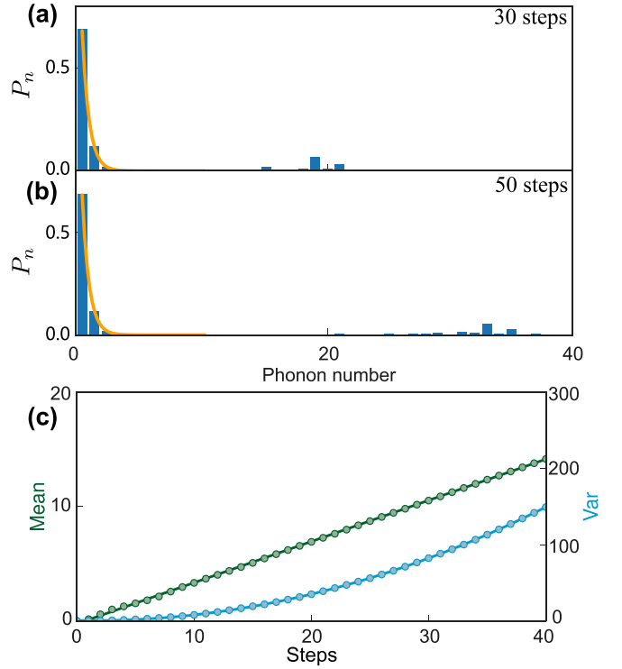
FIG. 6. Simulation result of the phonon-state distribution after (a) 30 and (b) 50 steps, with \theta_1 = \pi/2, \theta_2 = 0 , and \phi = 0 . A single E = 0 bound state appears, as predicted for the real bulk system in the phase (1,0), that has a different topology from the virtual bulk system. The histogram shows the phonon distribution and the orange line is the analytical solution of the eigenstate. (c) Mean and variance of the QW vs steps. The features of the quadratic increment of the deviation and the linear increment of the mean are the patterns of acceleration of the classical random walk.
