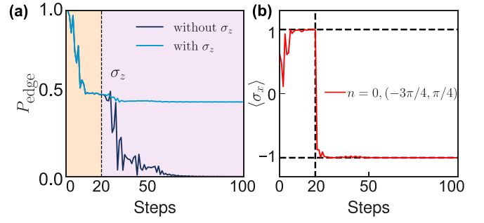
FIG. 12. Recovery of the bound state when the quench is between (1,0) and (0,1) with the same parameters as in Fig. 8(d). (a) Edge population P_{\text{edge}} vs evolution steps with and without \sigma_z operation at the end of step N_0 , which transfers |+\rangle to |-\rangle and thus helps recover the bound state. (b) Spin-state dynamics with the additional \sigma_z operation. We note how a \pi -energy bound state is built starting from a 0-energy bound state.
