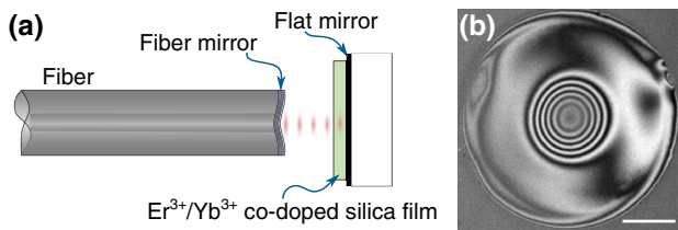
Fig. 1. Schematic of the FFPC for lasing. (a) The FFPC is formed by a concave fiber mirror and a flat mirror. An Er 3+ /Yb 3+ co-doped silica film (thickness of 35.1 \mu m) is set inside the cavity and bonded onto the flat mirror. (b) An interferometric image of the concave surface of the fiber mirror (with the scale bar of 30 \mu m), and the radius of curvature of the concave mirror is calculated as 100 \mu m from the concentric fringes.
