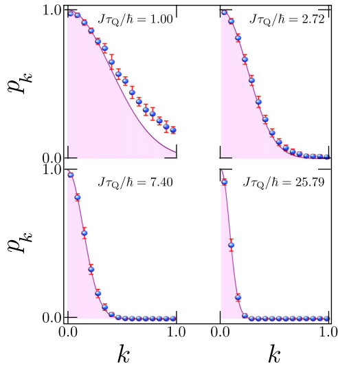
Fig. 2 Excitation probability in the ensemble of Landau-Zener crossings.
