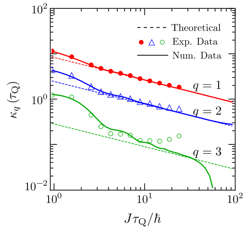
Fig. 4 Universal scaling of the cumulants \kappa_q(\tau_Q) of the kink-pair number distribution P(n) as a function of the quench time.
