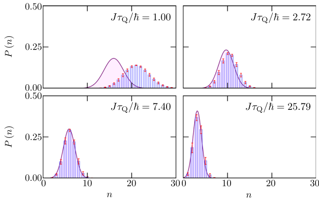
Fig. 3 Probability distribution of the number of kink pairs P(n) generated as a function of the quench time.
