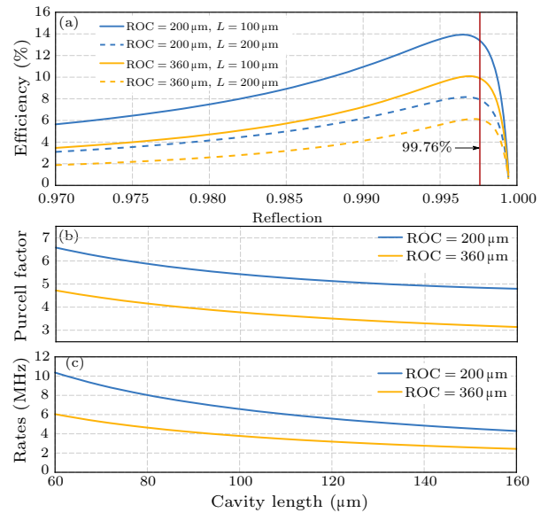
Fig. 4. Numerical simulation of the florescence enhancement of a trapped \text{Yb}^+ with an FFPC. Two cavities with ROC=360 \mu\text{m} (yellow lines) and ROC=200 \mu\text{m} (blue lines) are simulated. (a) Collection efficiency with the reflection of the output mirror. (b, c) The Purcell enhancement factor and photon emission rates into single fiber modes of FFPCs along with cavity length.
