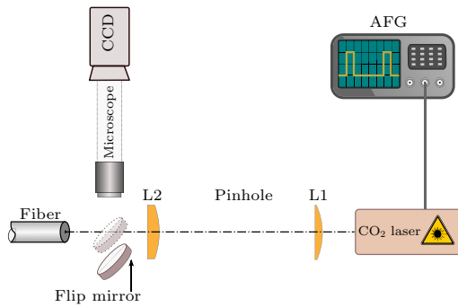
Fig. 1. Schematic diagram of laser machining setup for fabricating FFPCs. The pinhole is set on the focal plane of lens L1 as a spatial filter, L2 is an aspheric lens with a focal length of 50 mm, and the microscope is used to position the fiber core to the laser spot of L2 by the aid of the flip mirror.
