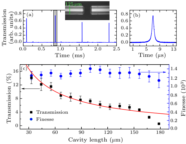
Fig. 3. Transmission measurement of the FFPC. (a) Transmission spectrum at 369 nm by scanning the cavity length over three free spectrum ranges. Inset: the cavity configuration. (b) Details of the second peak in (a). (c) The cavity finesse (blue dots) and total transmission efficiency (black cubes) versus the cavity lengths, and the red line is the simulated total transmission efficiency.
