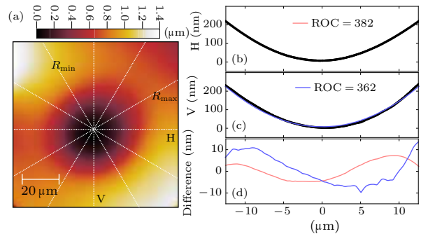
Fig. 2. Surface characterization of a typical machined fiber. (a) Mirror profile with an area of 90\text{ }\mu\text{m} \times 90\text{ }\mu\text{m} measured by an AFM. (b, c) Horizontal (H) and vertical (V) section of the dashed square of (a), black: section data, red (blue): circle fit of H (V). (d) Difference between data and fit in (b) and (c).
