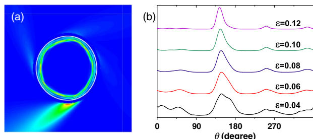
Fig. 3. (Color online) (a) Typical near-field profile of clockwise traveling WGM. The field outside of the cavity is enhanced for visualization. (b) Far-field patterns of WGMs for different deformations by Boundary Element Method simulated wave function.
