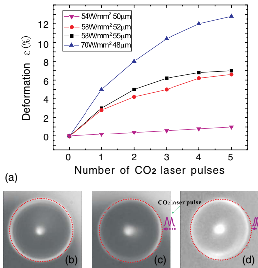
Fig. 1. (Color online) (a) Measured deformation with different \text{CO}_2 pulse intensity and number. The legend shows the laser power and microsphere diameter for each line. (b)–(d) Top views of the same microsphere variation with 0, 2, and 5 \text{CO}_2 laser pulses from the arrow direction, respectively. The sphere diameter is about 50 \mu\text{m} .
