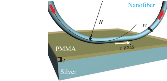
Fig. 1. Schematic diagram of the hybrid plasmonic waveguide, consisting of a bending nanofiber on a metal substrate, which is covered by a thin PMMA film (thickness t ).
