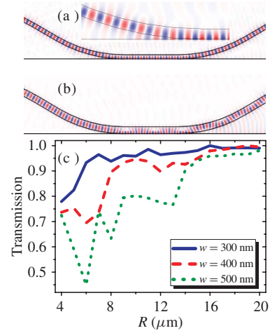
Fig. 2. (a) and (b) Filed distributions for w = 300 -nm and w = 500 -nm waveguide, respectively, with R = 10 \mu m and t = 0 . (c) Transmission of the hybrid waveguide for different w and R , with t = 0 . Inset: the detail of adiabatic conversion
