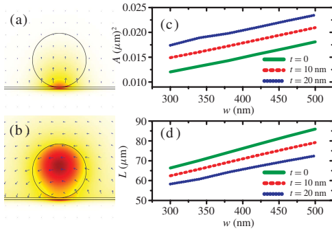
Fig. 3. (a) Energy density distribution at the cross section of the hybrid waveguide for the TE mode. (b) TM mode with w = 300 nm and t = 10 nm. The arrows indicate the directions of electric field. (c) Mode area. (d) Propagation length of the hybrid plasmonic mode (a) with t = 0, 10, 20 nm for various waveguide widths.
