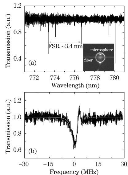
Fig. 1. (a) Typical transmission spectrum of a silica microsphere with a diameter of 39 \mu\text{m} . The transmission dips correspond to the WGM resonances. Inset: the optical image of microsphere coupling with a low-loss fiber taper. (b) Enlarged mode spectrum at 780 nm measured at sweeping speed d\nu(t)/dt = 12.5 \text{MHz}/\mu\text{s} and input power \sim 2 \mu\text{W} . The smooth line represents the theoretical calculation with Q_0 = 2.3 \times 10^8 and Q_{\text{ex}} = 14.3 \times 10^8 .
