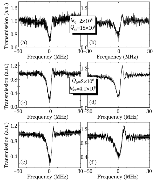
Fig. 3. Slow and fast scanning experimental results and theoretical calculation (smooth lines) for different coupling regimes. For the theoretical calculations, Q_0 and Q_{\text{ex}} are used with (a), (b) 2 \times 10^8 , 18 \times 10^8 ; (c), (d) 2 \times 10^8 , 4.1 \times 10^8 ; (e) 4 \times 10^8 , 1.1 \times 10^8 ; and (f) 5 \times 10^8 , 0.7 \times 10^8 , respectively. The left column corresponds to the sweeping speed d\nu/dt = 12.5 \text{ MHz}/\mu\text{s} , while the right column corresponds to 25 \text{ MHz}/\mu\text{s} . The excitation power used is 2 \mu\text{W} when the thermal effect is negligible.
